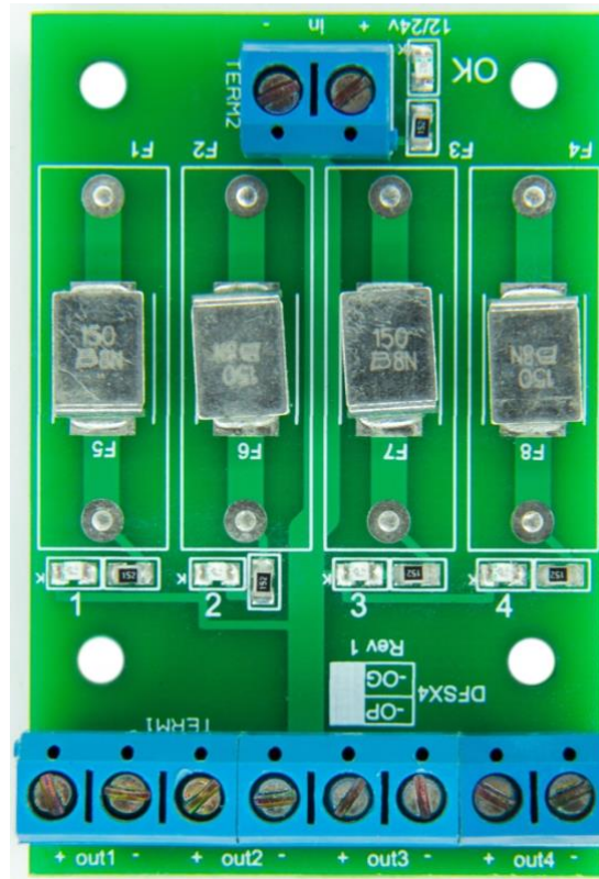
DFX4-OP 4-way, self-resetting, electronically-fused output splitter
